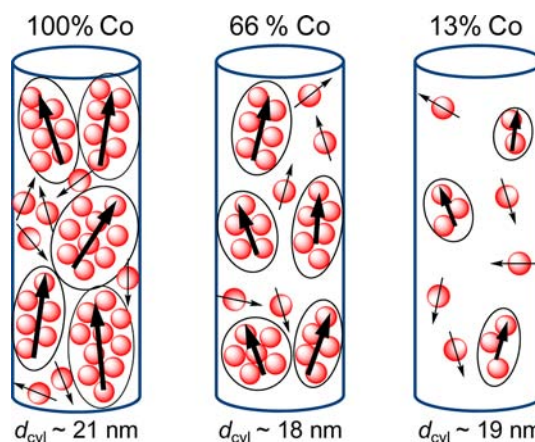
Figure 8. Schematic illustrating the decreased dipolar interactions between cobalt nanoparticles with decreasing cobalt density in the cylindrical domains. By controlling the number of cobalt units in the BCP primary sequence, the density of cobalt atoms in the nanocylinders is controlled. As the density decreases, the number of cobalt nanoparticles is decreased. This results in a larger average spacing between particles since the cylinder diameter is held constant. By increasing the average spacing between particles, the dipolar interactions between cobalt nanoparticles (represented by the ovals) become weaker, 22 leading to lower magnetic reversal temperatures.
