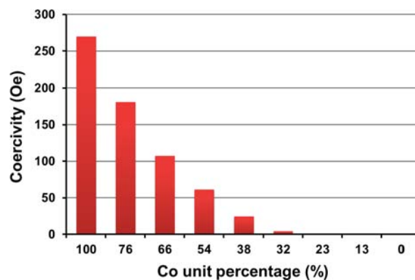
Figure 5. Impact of decreasing the Co unit percentage in the cylindrical domains on the coercivity of the nanostructured BCP materials.
