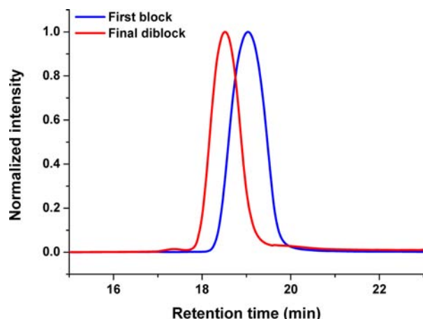
Figure 2. Representative GPC curves for the first block composed of the C_{16} homopolymer (blue) and the final C_{16} - b -(Co- r -Fe) diblock copolymer (Poly5) (red).
