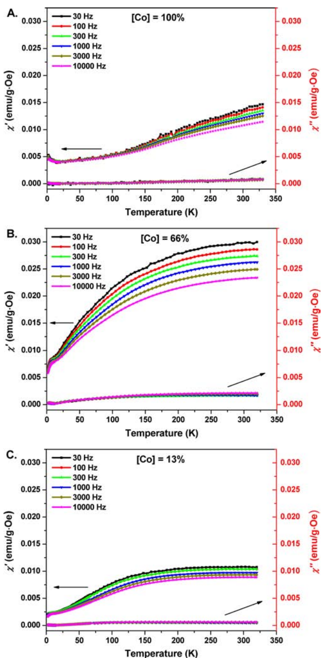
Figure 7. Temperature dependence of the in-phase and out-of-phase components, \chi' and \chi'' , of the AC susceptibility, measured at various frequencies (30–10000 Hz) with an AC field of 5 Oe, for the nanostructured BCP materials with (A) 100%, (B) 66%, and (C) 13% Co units in the cylindrical domains.
