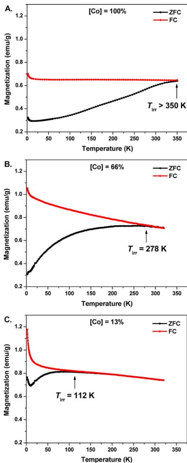
Figure 6. ZFC and FC magnetization curves under an applied field of 100 Oe for the nanostructured BCP materials with (A) 100%, (B) 66%, and (C) 13% Co units in the cylindrical domains. The irreversible temperatures ( T_{\text{irr}} ) for the samples are indicated on the plots.
