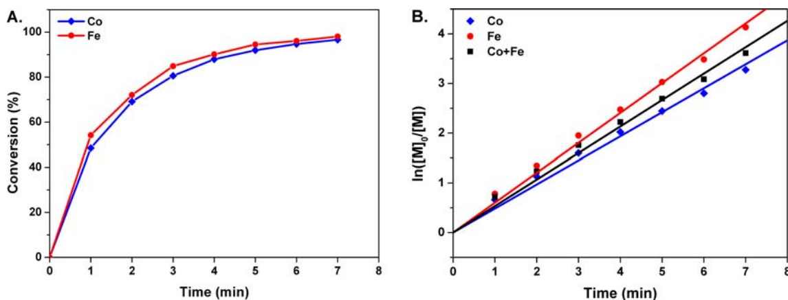
Figure 3. (A) Conversion of the cobalt complex-functionalized (Co) monomer 4 (blue) and the ferrocene-functionalized (Fe) monomer 5 (red) as a function of time for the random copolymerization of monomers 4 and 5. (B) Linear fits of the first-order time–conversion relation of the Co monomer 4 (blue), Fe monomer 5 (red), and the sum of 4 and 5 (black). All the R^2 values for the linear fits are around 0.98. [\text{M}] denotes the monomer concentration.
