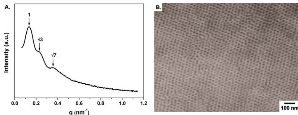
Figure 4. Representative (A) SAXS curve and (B) TEM micrograph of a block-random copolymer (Poly5) after solvent annealing in chloroform.
